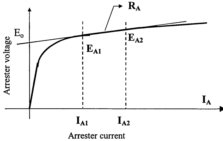
Figure 9—Arrester characteristics
